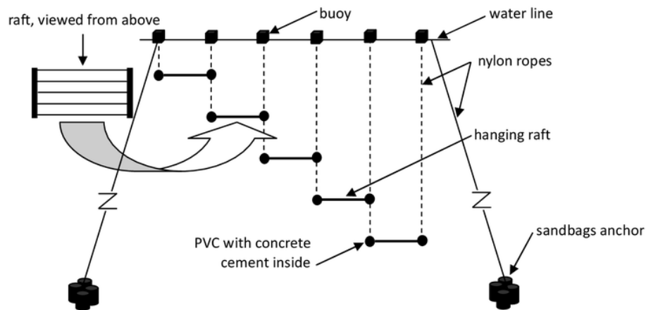
Figure 1. Hanging rafts construction, viewed from frontage (Wenno 2014).
